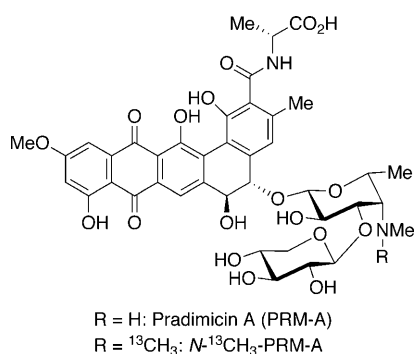
Scheme 1. Structures of pradimicin A (PRM-A) and N\text{-}^{13}\text{CH}_3\text{-PRM-A} .
